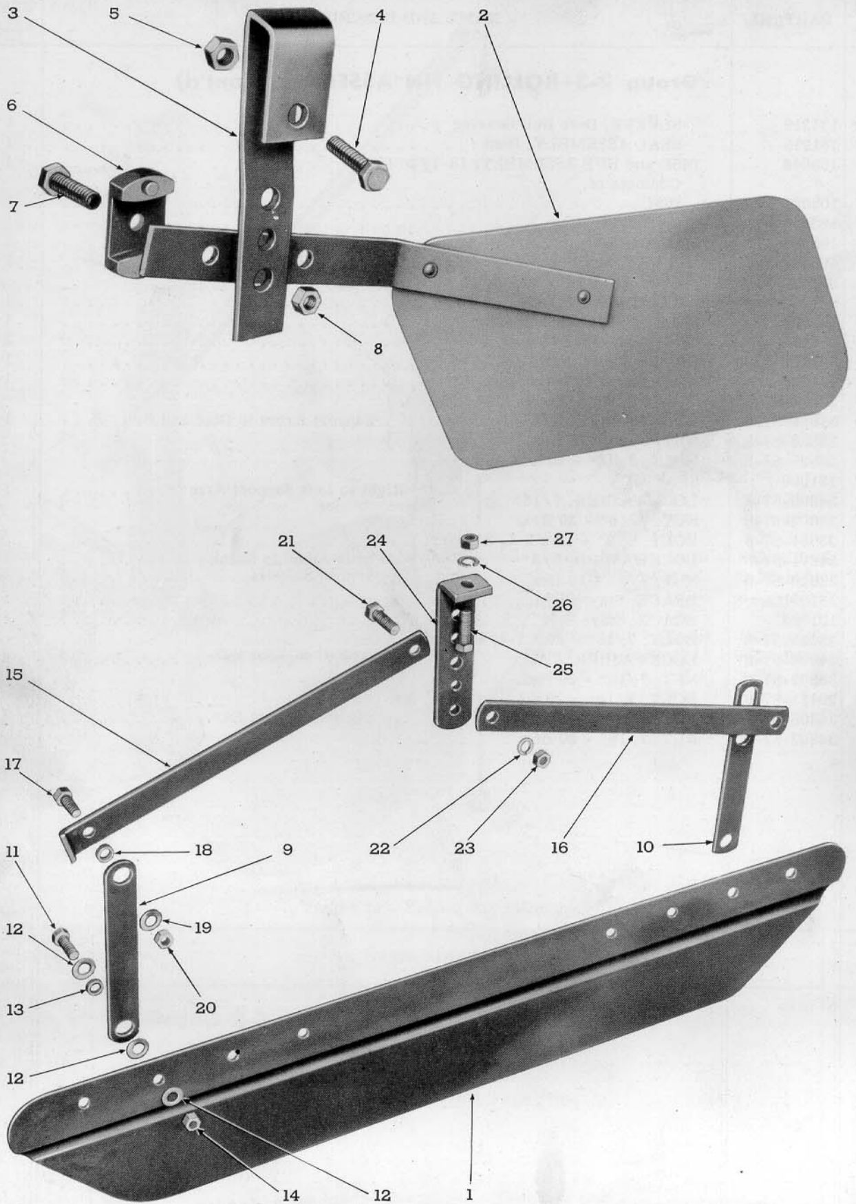
Figure 14 - Shield Assemblies
