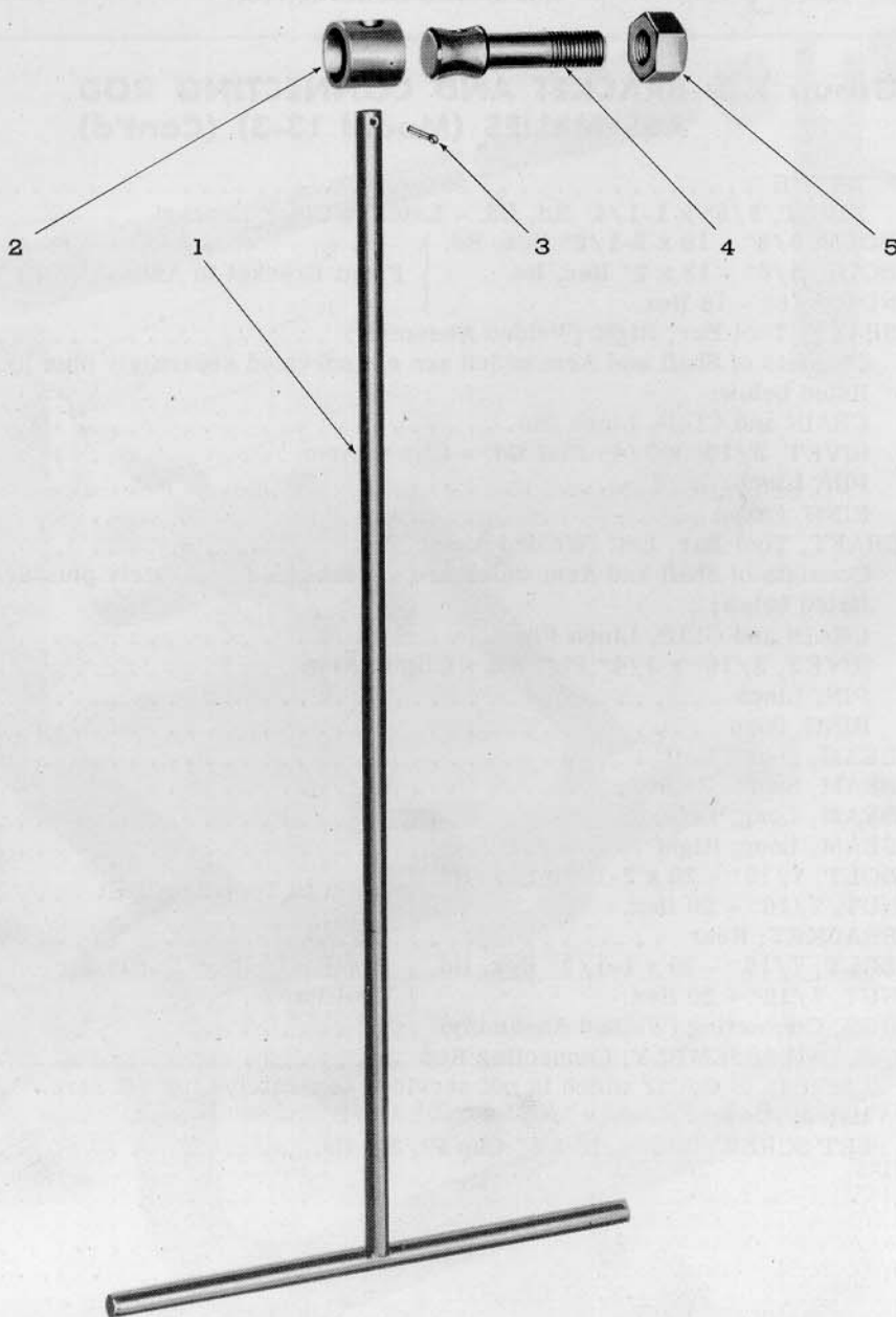
Figure 16 - Steering Pointer Assembly
