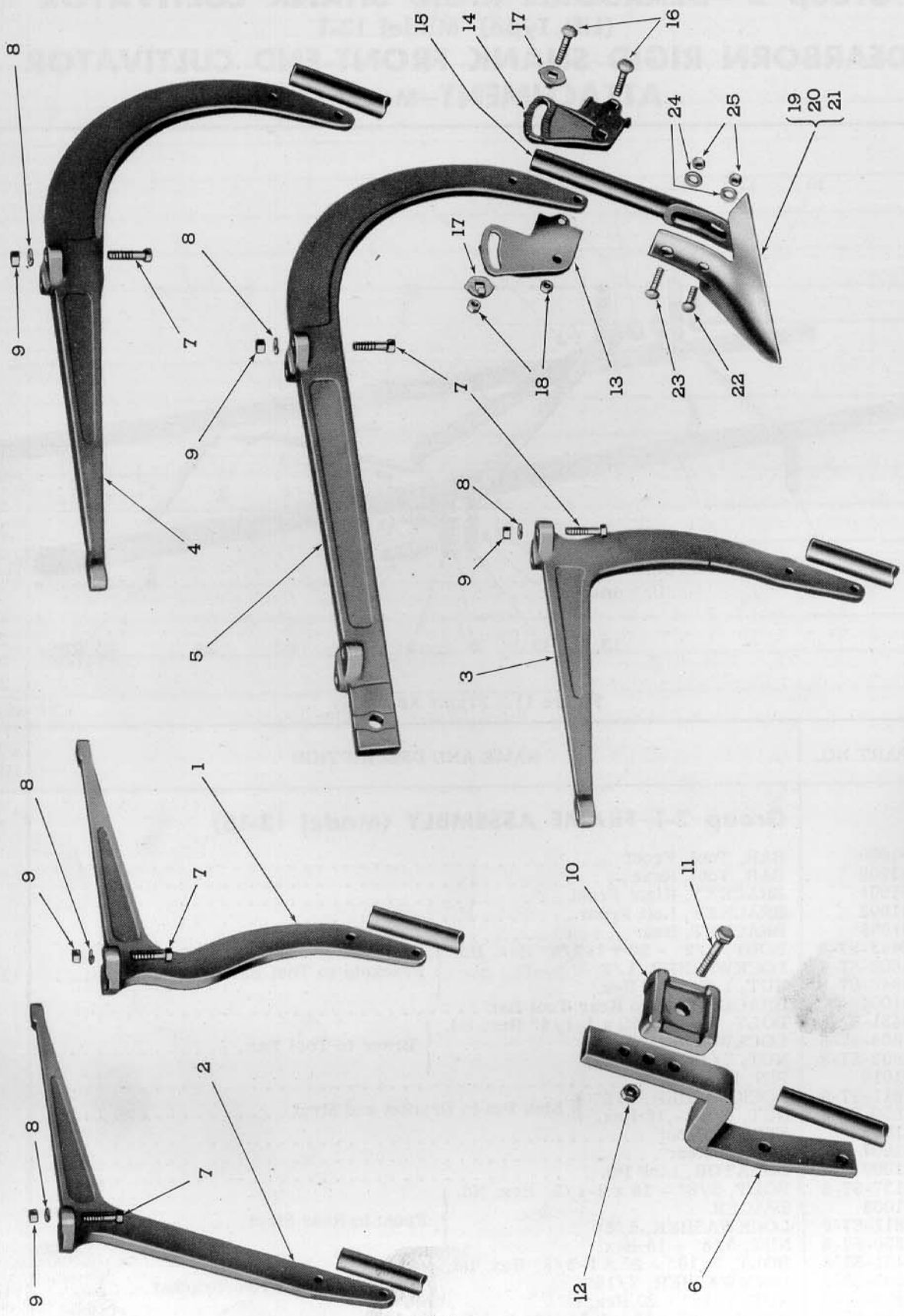
Figure 12 - Shank Assemblies
