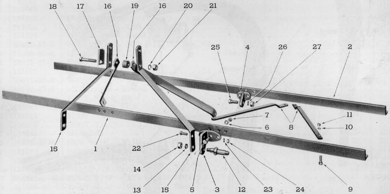
Figure 11 - Frame Assembly
