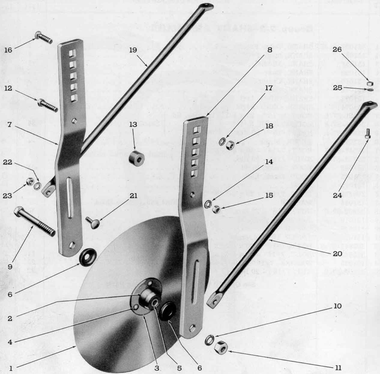
Figure 13 - Rolling Fin Assembly
